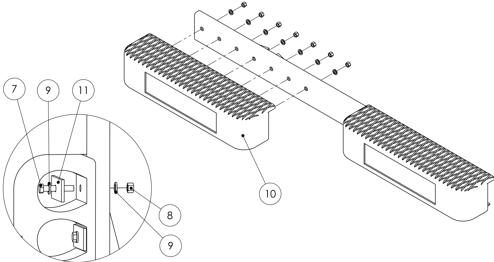
Hardware Mounting
